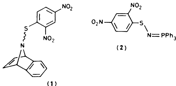
Figure. Molecular structure of compound (2) showing the atom numbering scheme
