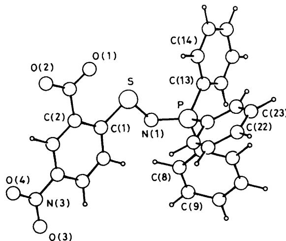
Figure. Molecular structure of compound (2) showing the atom numbering scheme
